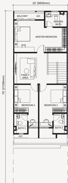
First Floor
